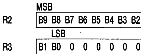
D OUT from LTC1095 stored in 8051 RAM
