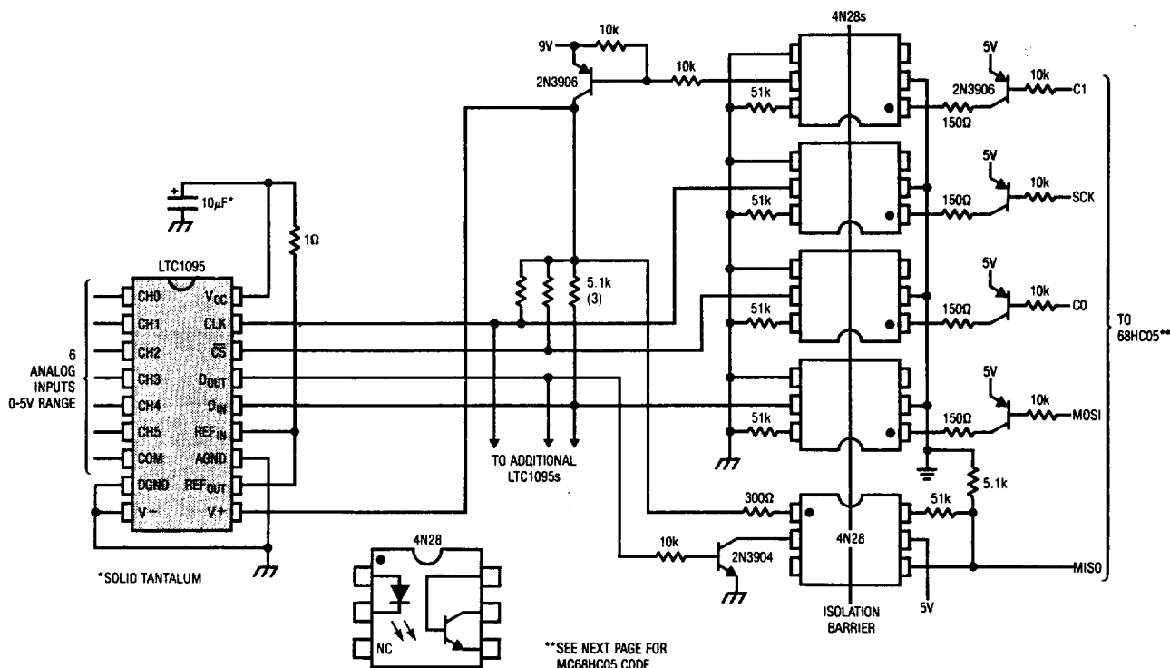
Micropower, 500V Opto Isolated, Multichannel, 10-Bit Data Acquisition System
