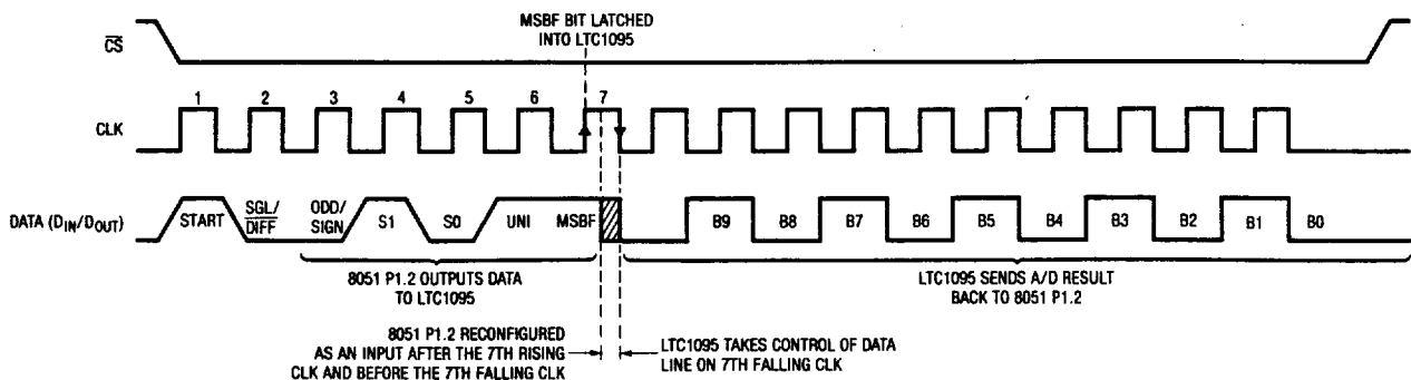
Data Exchange Between LTC1095 and 8051
