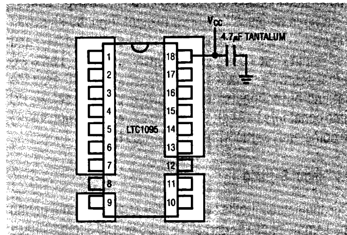
Figure 4. Example Ground Plane for the LTC1095
