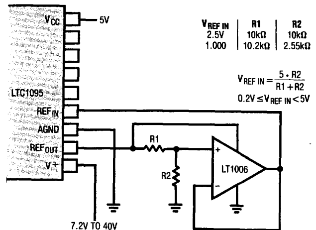
Figure 17. Operating LTC1095 on Reduced Reference Voltage
