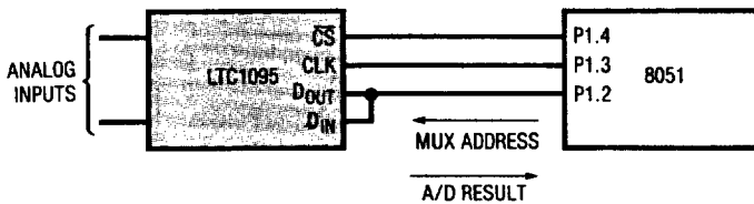
D OUT from LTC1095 stored in 8051 RAM
