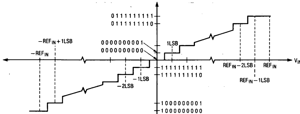
Bipolar Transfer Curve (UNI = 0)
