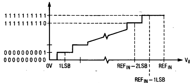
Unipolar Transfer Curve (UNI = 1)
